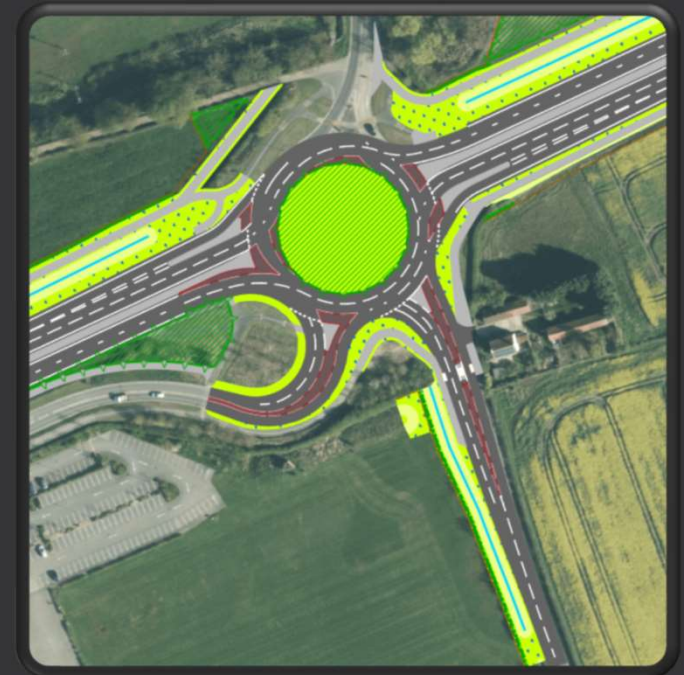
Wigginton Road Roundabout – Proposed Works
