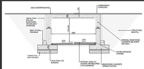
Typical Cross Section Through Proposed Underpass at Strensall Road Roundabout
