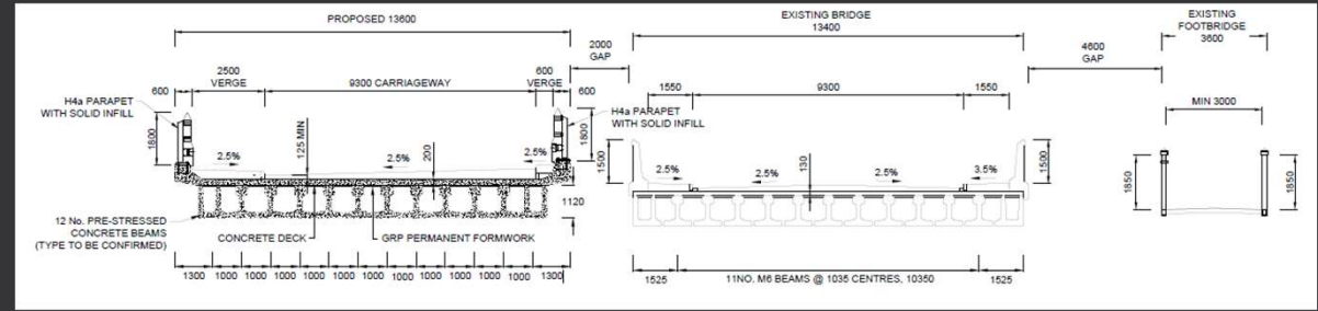
Typical Cross Section Through Existing and Proposed Bridges over York – Scarborough Railway Line
