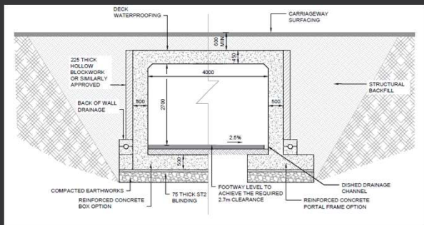
Typical Cross Section Through Proposed Clifton Moor Underpass
