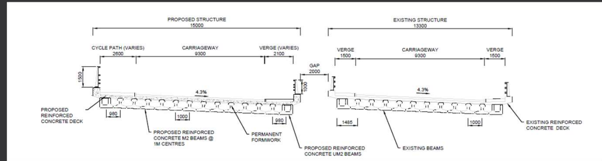
Typical Cross Section Through Existing and Proposed Bridges over York – Scarborough Railway Line
