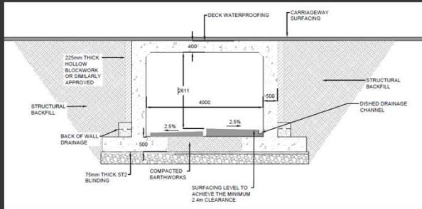
Typical Cross Section Through Proposed Haxby Roundabout Underpasses
