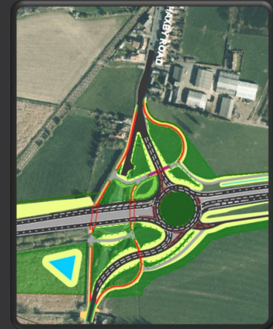
Haxby Road Roundabout – Proposed Works
